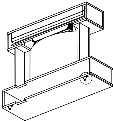
Fasten bracket to bottom of hearth section, and fasten to wall underneath.
